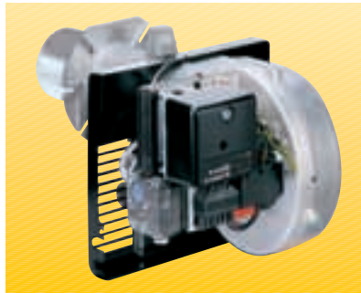
In GS10 and GS20 models the control box is separated from the ignition transformer
