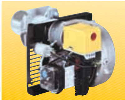
Control box fitted with an ignition transformer in GS3 and GS5 models
